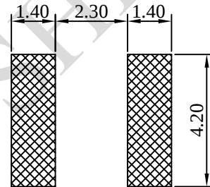
( PCB Pattern )
